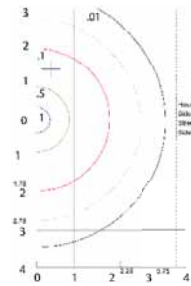
40W Flat (Full-Cutoff Lens) Max Candela: 811 at 55° Angle .01 fc at over 3 25' mtg htgs. B1-U0-G1. ITL75688.
