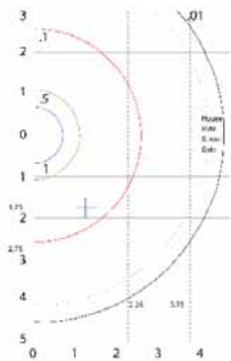
70W Dome Lens: Max Candela: 1445 at 65° Angle .01 fc at >4 25' mtg htgs B3-U2-G2. Final Tests Pending
