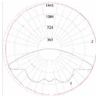
70W Dome Lens: Max Candela: 1445 at 65° Angle .01 fc at >4 25' mtg htgs B3-U2-G2. Final Tests Pending
